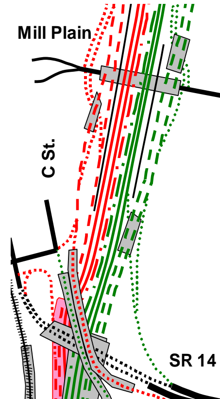
Concept: 6 through, 4-6 aux lanes
