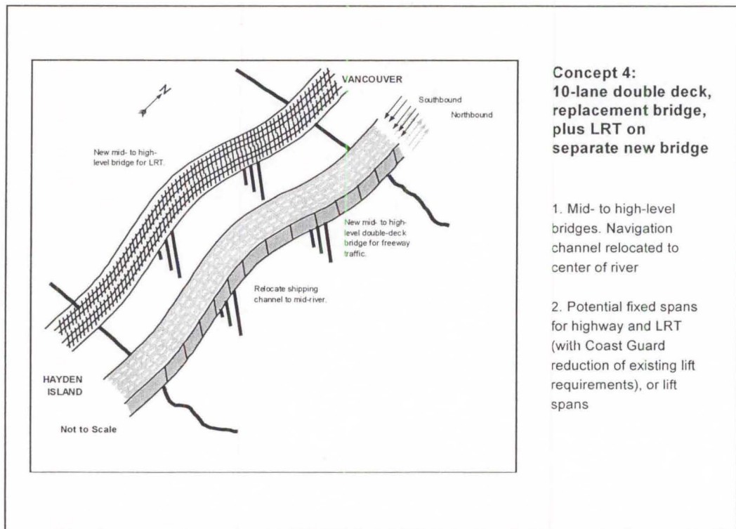
Figure 4: Bridge Concept 4
