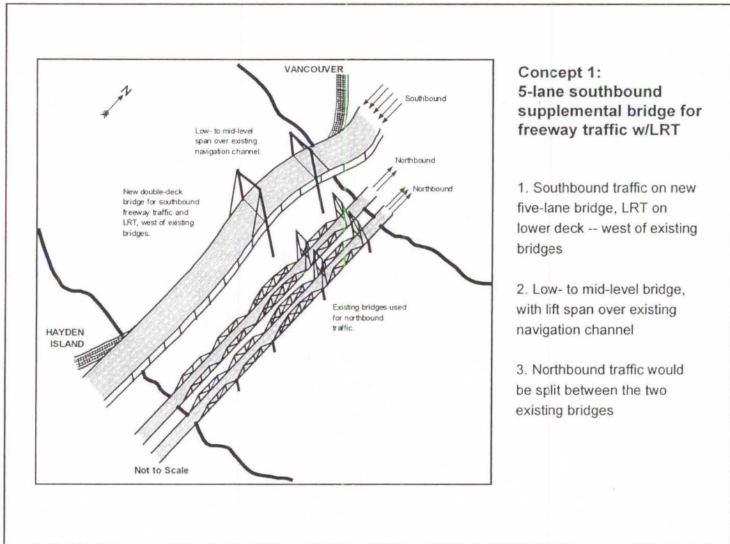
Figure 3: Bridge Concept 1
