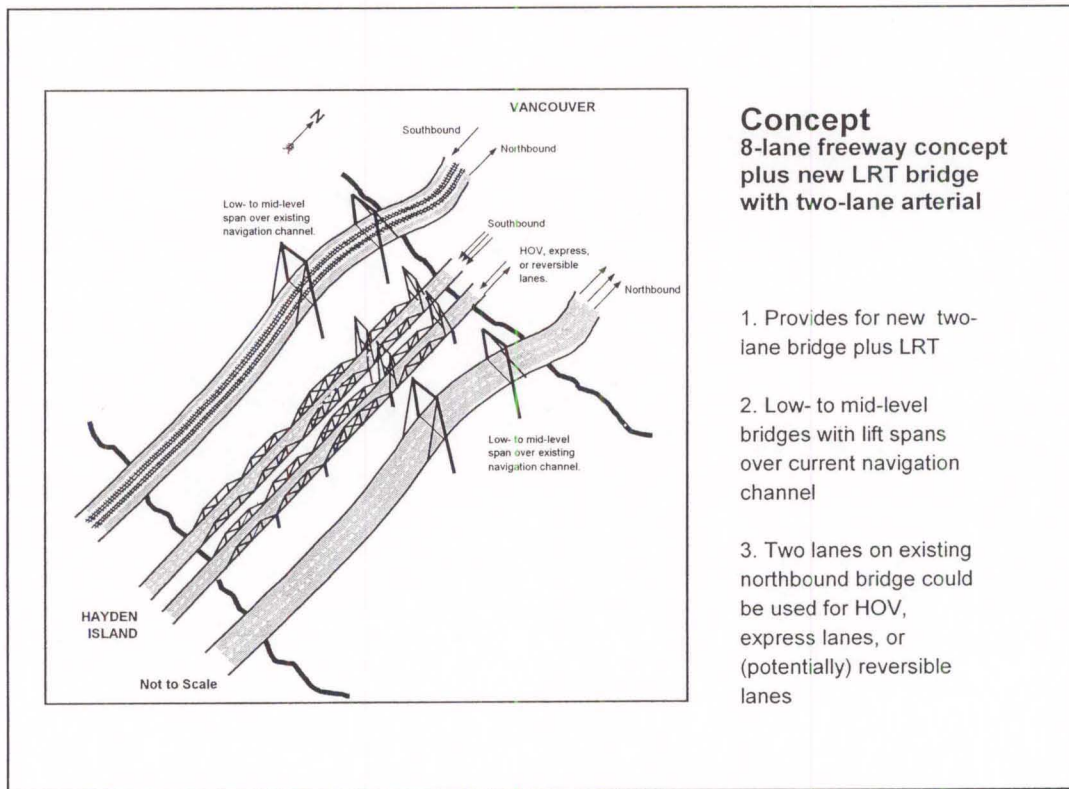
Figure 6: Bridge Concept 7
