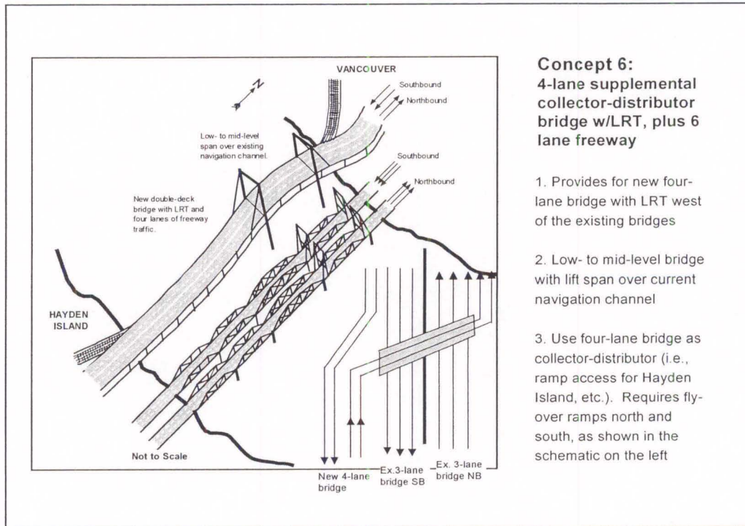
Figure 5: Bridge Concept 6
